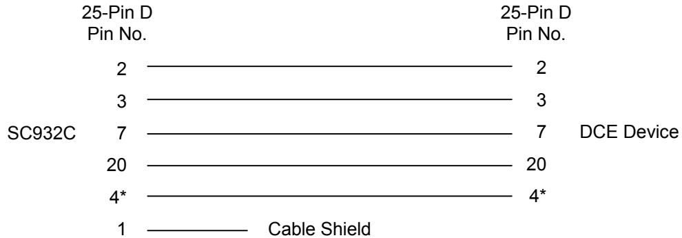
FIGURE A-1. Minimum Connections for SC932C to 25-pin DCE Interface
