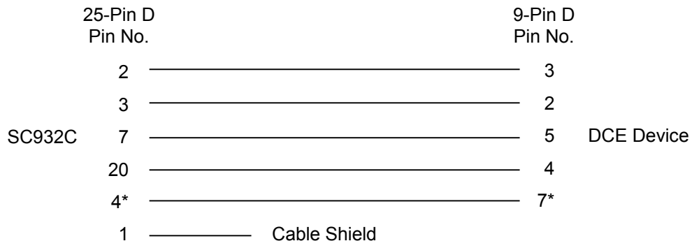
FIGURE A-2. Minimum Connections for SC932C to 9-pin DCE Interface
