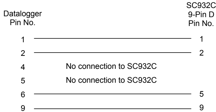
FIGURE B-1. Connections for Using SC932C in 'Printer' Mode
