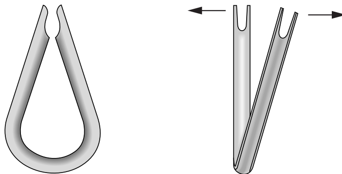
FIGURE 2-7. Thimble Twisting
