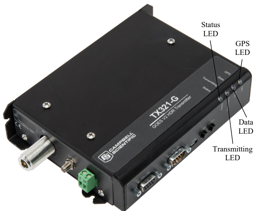
FIGURE 7-1. TX321 LEDs
