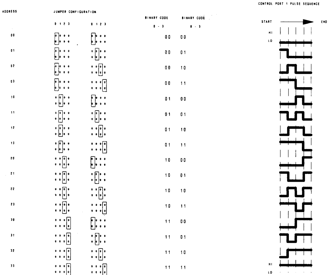
FIGURE 1B. Address Jumper Identification
