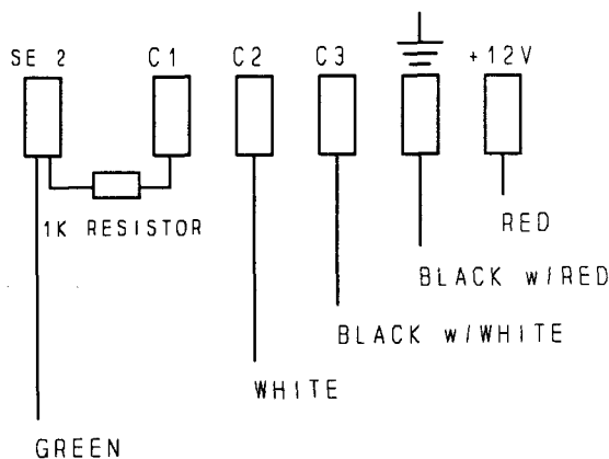
WIRING DIAGRAM FOR 21X
