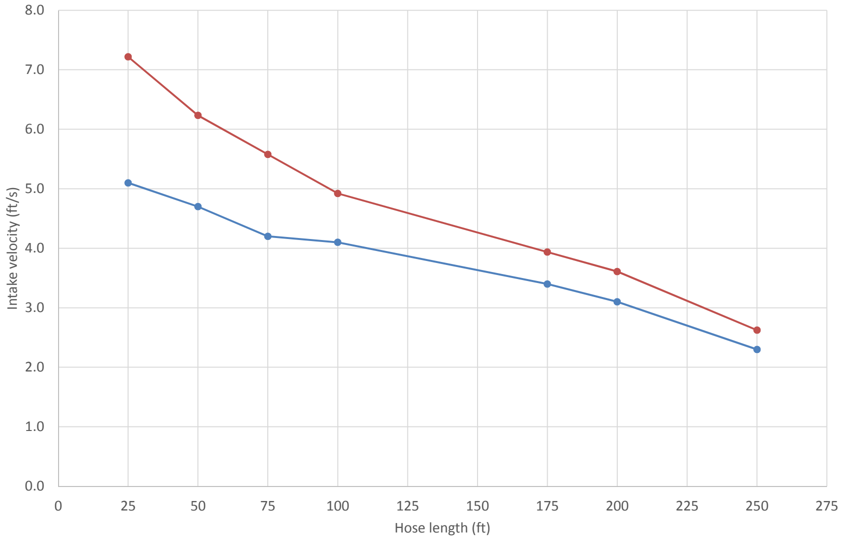
Standard and large pump intake velocities as a function of hose lengths
