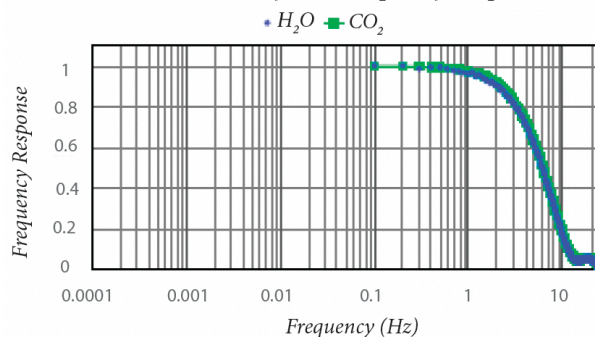
CPEC300-Series System Frequency Response
